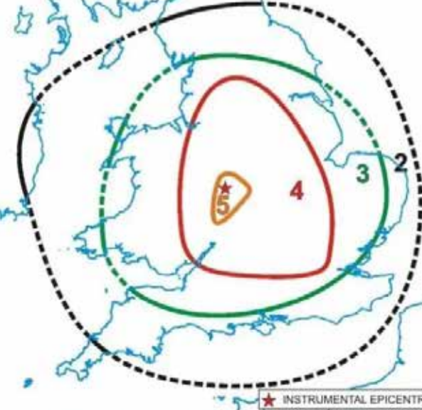
Intensity Vs Magnitude of Earthquake
