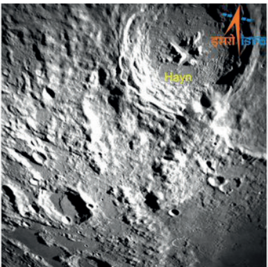
Lunar far side area as imaged from the Lunar Hazard Detection and Avoidance Camera (LHDAC) onboard Chandrayaan-3 on August 19, 2023
