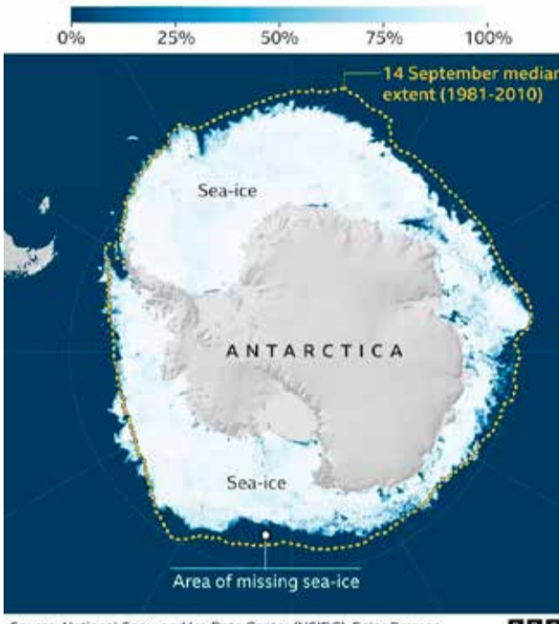
Winter sea-ice is missing in some areas. Sea-ice concentration, 14 September 2023.
