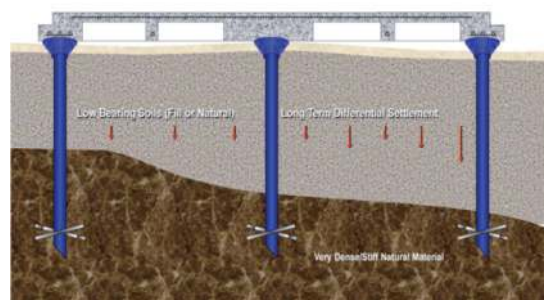
Typical slab on screw pile footing for ‘P’ sites
