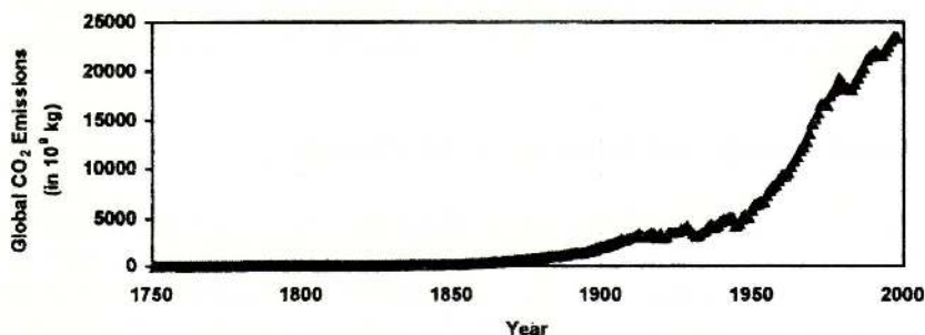
Figure 1: Global CO 2 emissions from the burning of fossil fuels and the manufacture of cement.
