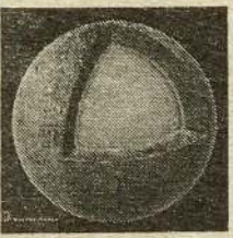
Mercury
