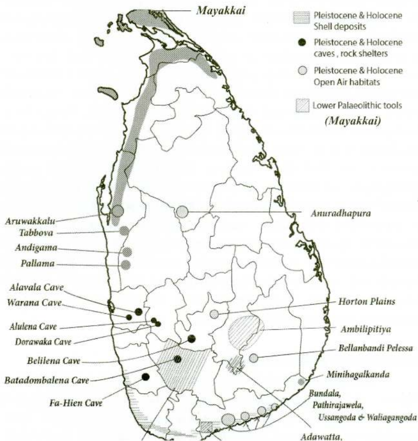
A representation of some of the important palaeobiodiversity sites of Sri Lanka (Kelum Manamendra - Arachchi)
