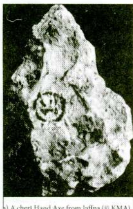
a) A chert Hand Axe from Jaffna (© KMA)
