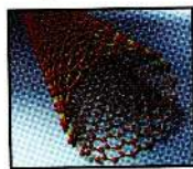
Nano tubes
