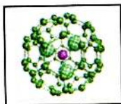
Bucky ball
