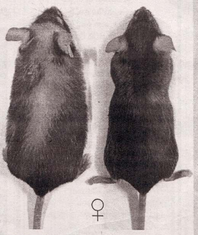
Old //11+/+ Old //11-/-
