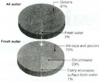
The global distribution of the earth's water resources
