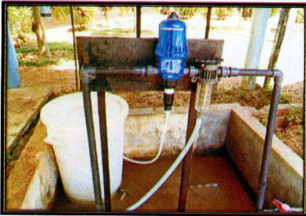
Chlorination Pump
