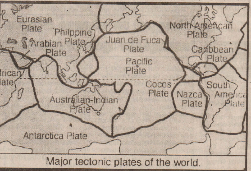
Major tectonic plates of the world.
