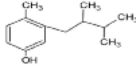
3-(2,3-dimethylbutyl)-4-methylphenol
