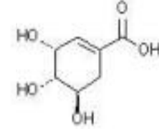
8 Stereoisomers
