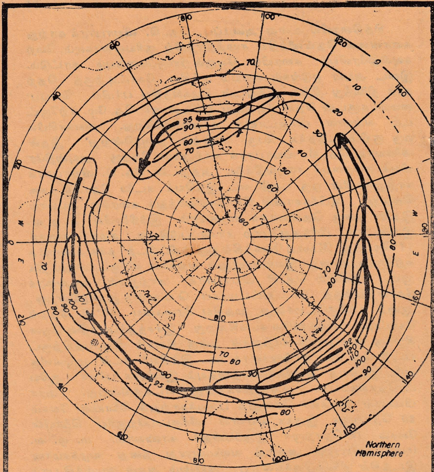
January MEAN POSITION AND STRENGTH of the JET STREAM (after NAMIAS and CLAPP)
