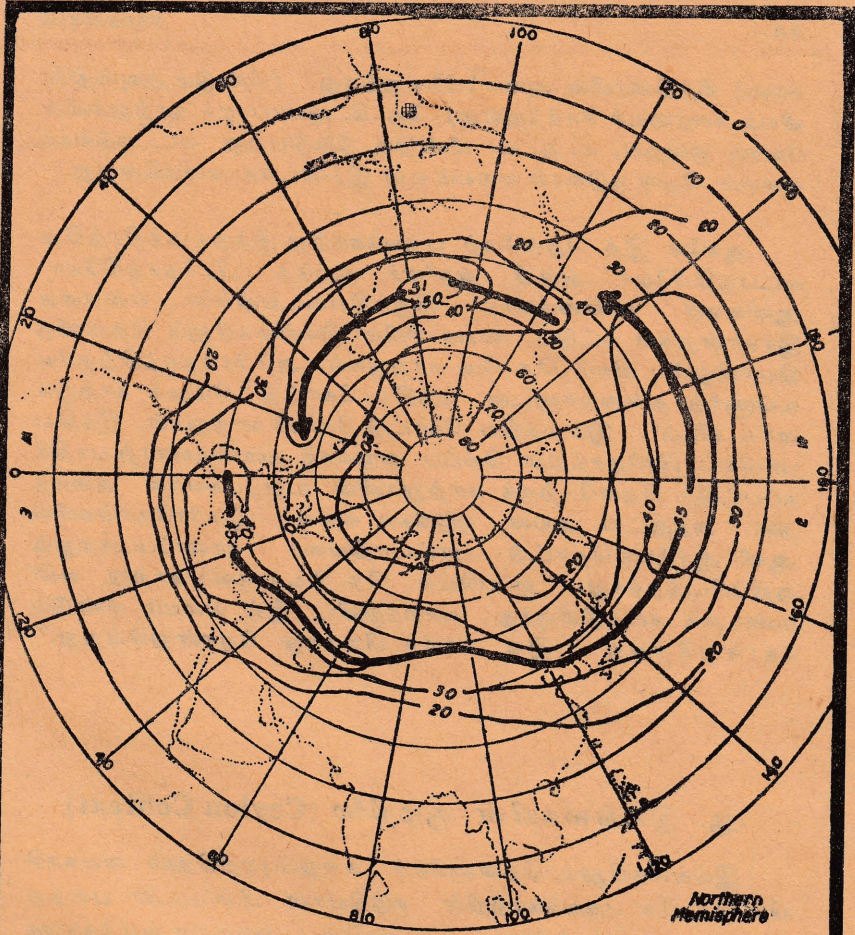
July MEAN POSITION and STRENGTH of the JET STREAM (after NAMIAS and CLAPP)
