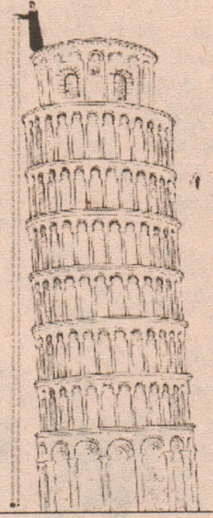
A. Galileo's Leaning Tower of Pisa Experiment
