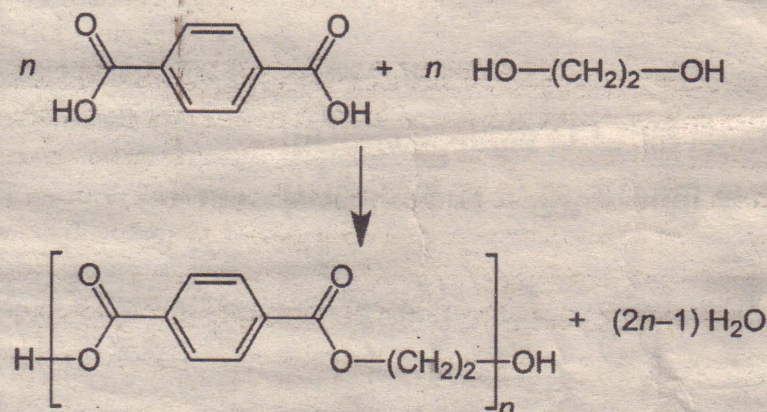
Polycondensation reaction in the production of PET
