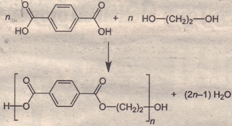
Polycondensation reaction in the production of PET
