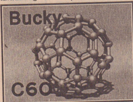
Bucky ball
