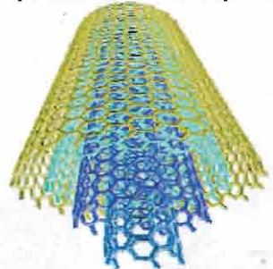
Carbon nano-structure
