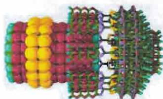
Molecular machinery
