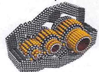
Molecular gears
