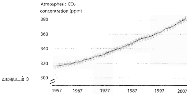
Figure 3: Atmospheric concentrations of carbon dioxide (CO 2 ) between 1957 and 2007
