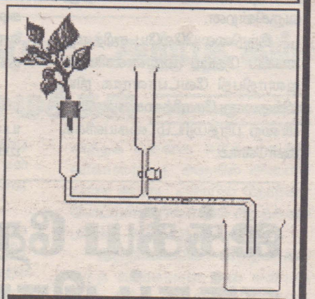
Ganong's Potometer
