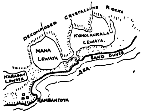
4. HAMBANTOTA LAGOONS SCALE 1 in = 2 MILES
