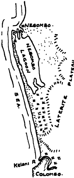
3. NEGOMBO LAGOON SCALE 1 in = 8 MILES
