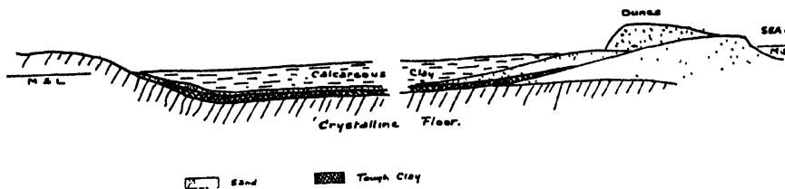
Fig. 3. A generalized diagram of a section across a typical lagoon.
