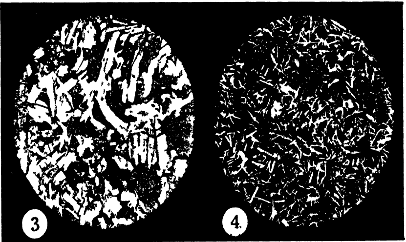
DYKE ROCKS
