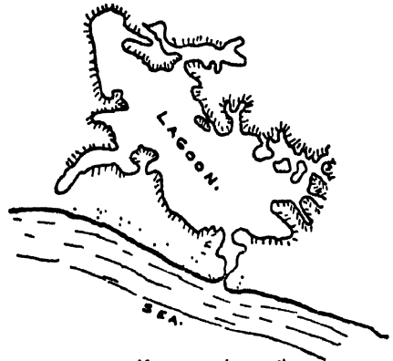
2. KOGGALA LAGOON. SCALE 1 in = 2 MILES
