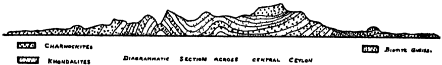
Fig. 6. Diagrammatic section across Central Ceylon.
