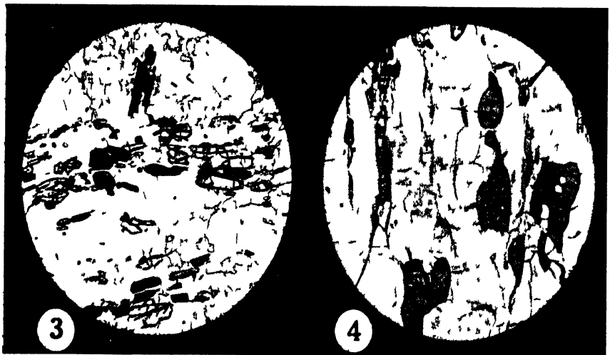
KHONDALITES AND AFFINE ROCKS
