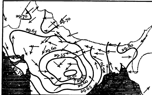
FIG. 17.—WEATHER CHART FOR 10 A.M., 10th September 1882.
