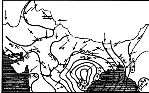
FIG. 16.—WEATHER CHART FOR 10 A.M., 8th September 1882.
