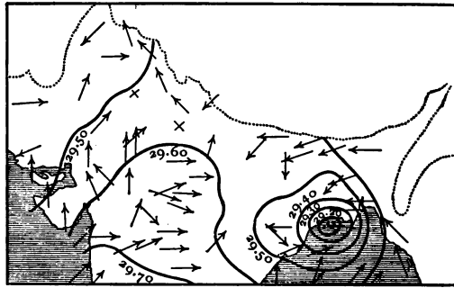
FIG. 20.—WEATHER CHART FOR 10 A.M., 29th June 1883.
