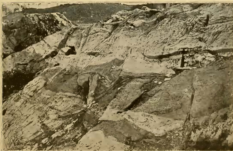
FIG. 2.—FOLIATION IN ROCKS OF THE GALLE GROUP. (Charnockite series.) Galle Fort. About 7 feet thickness shown.
